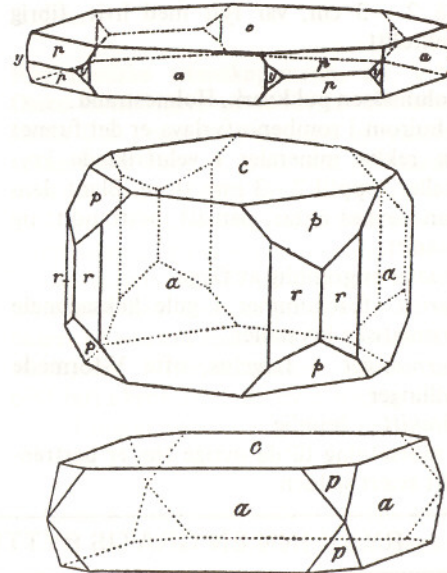
Ditolitt-gangen – Tafjord-tunnelen (over) Apophyllitt – Tafjord-tunnelen (under).
