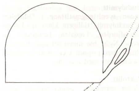
Ditolitt-gangen – Tafjord-tunnelen (over) Apophyllitt – Tafjord-tunnelen (under).
