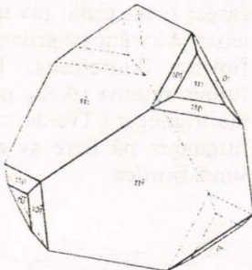
Helvin
