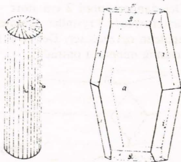
Astrophyllitt
