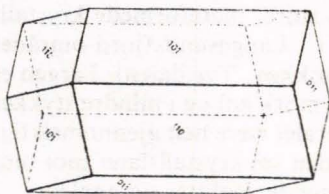
Sodalitt
